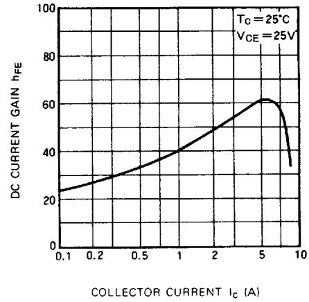
DC CURRENT GAIN VS. COLLECTOR CURRENT CHARACTERISTICS
